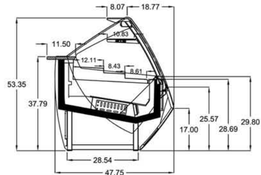
A45 PLAN VIEW & SIDE VIEW
